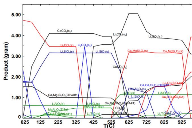
Figure 2. Modelling of the production for \text{Li}_4\text{SiO}_4 using BF slag.
