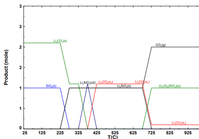
Figure 1. Modelling of the production for \text{Li}_4\text{SiO}_4 using \text{SiO}_2 .
